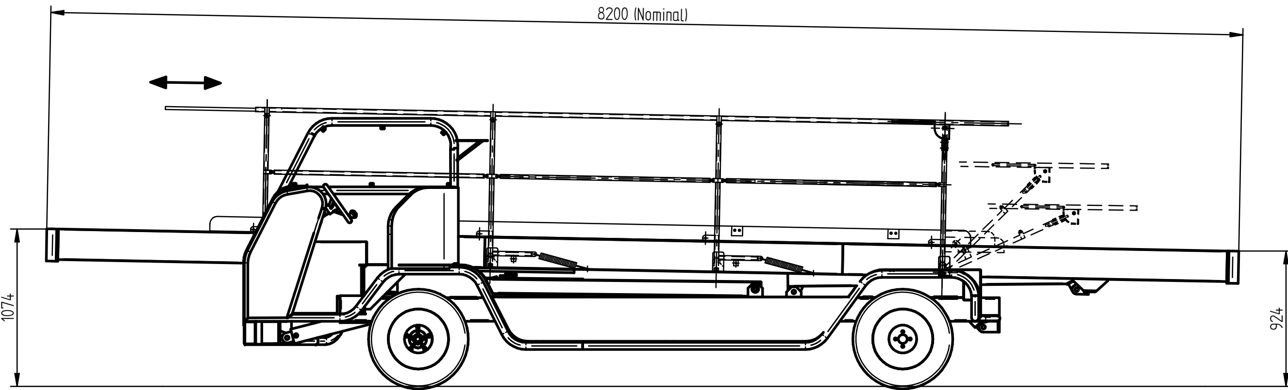
REAR RAM FULLY RETRACTED,FRONT RAM FULLY RETRACTED
