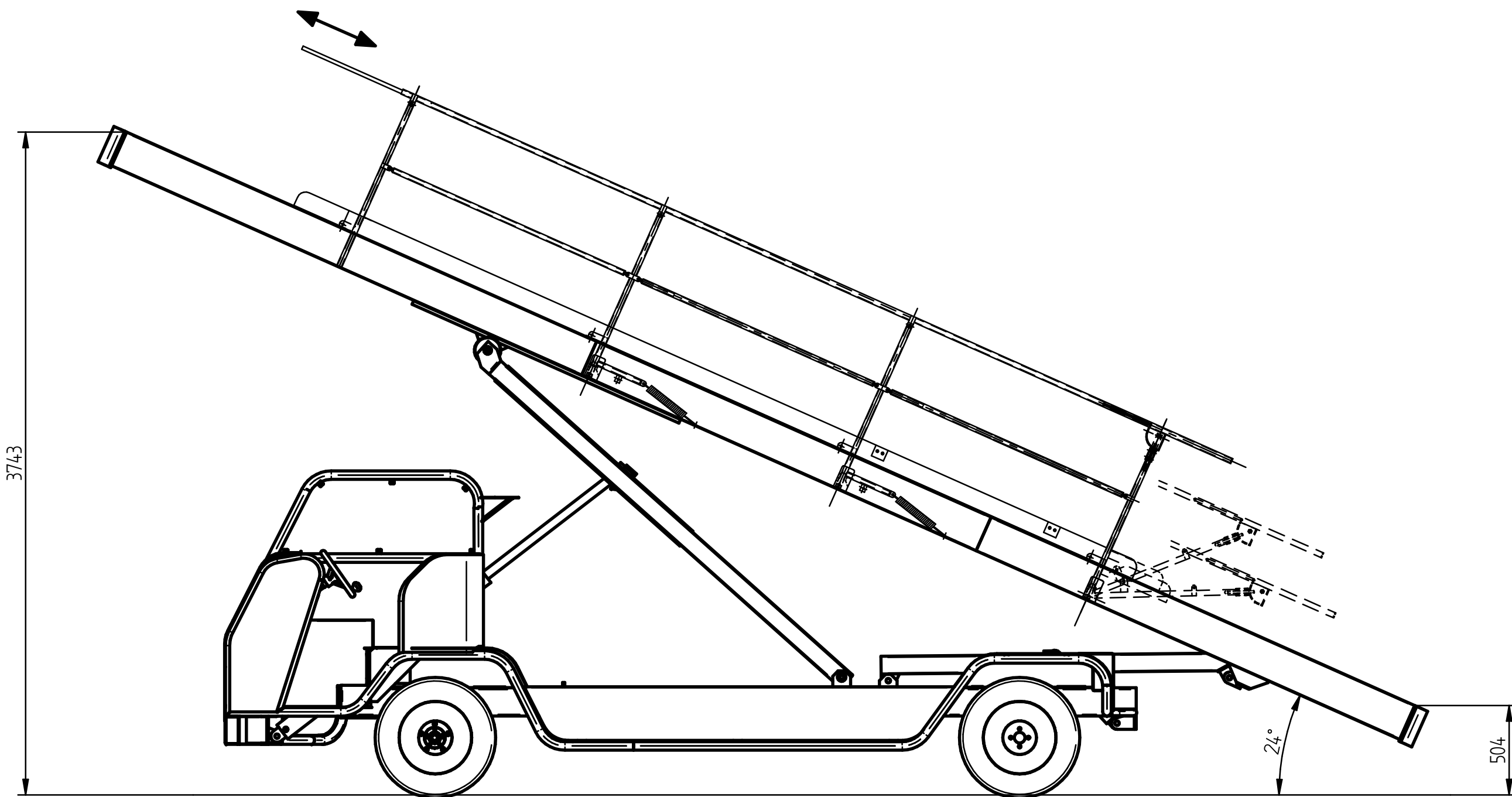
REAR RAM FULLY RETRACTED,FRONT RAM FULLY EXTENDED
