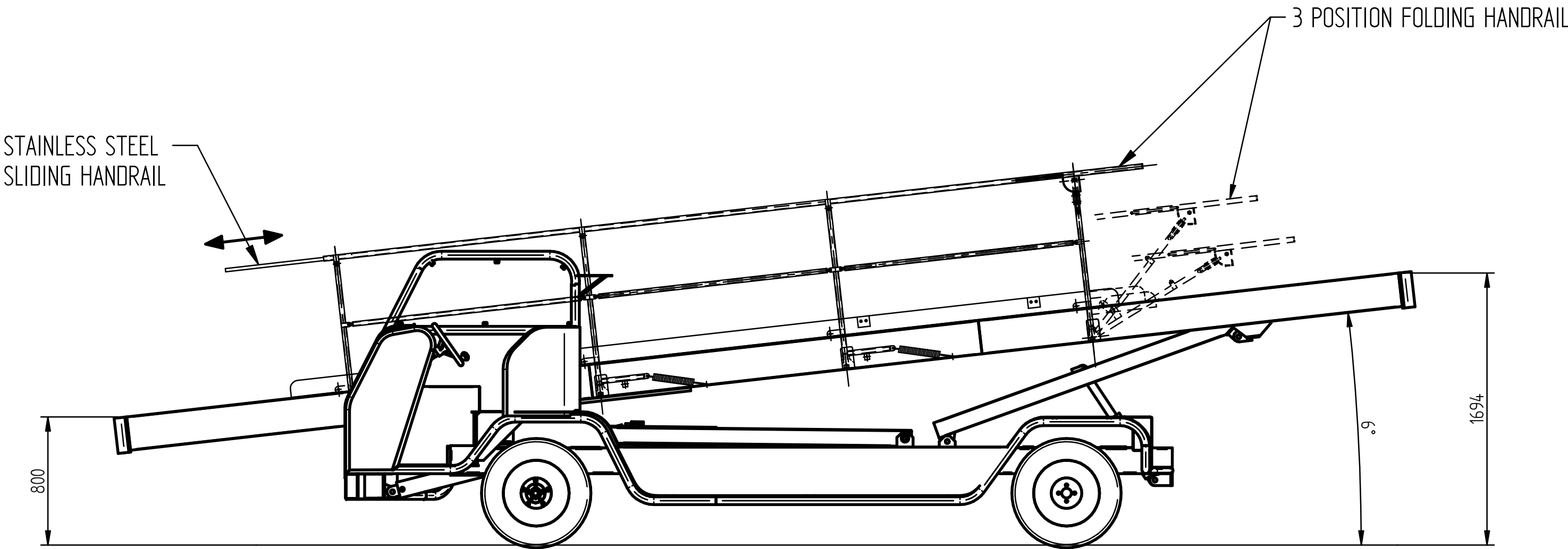
REAR RAM FULLY EXTENDED,FRONT RAM FULLY RETRACTED
