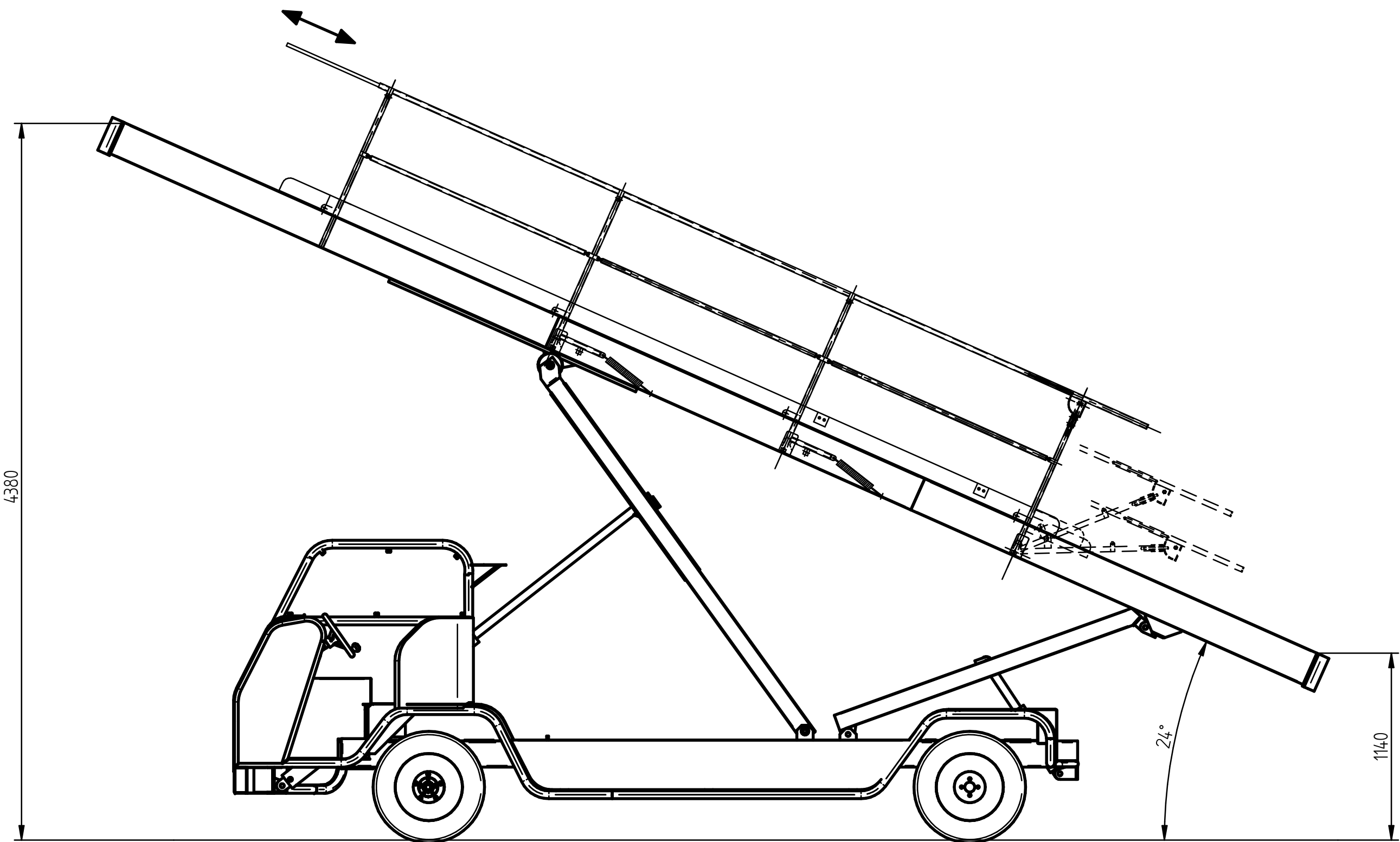
REAR RAM FULLY EXTENDED,FRONT RAM FULLY EXTENDED
